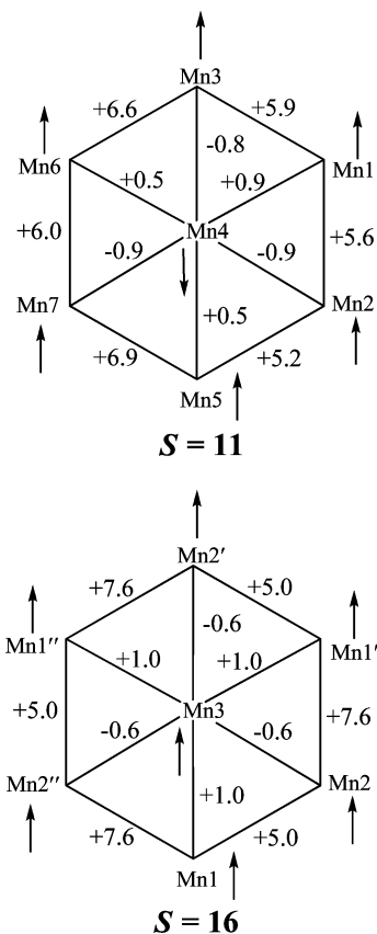
Figure 3. Calculated J values obtained by DFT of the anions of 1 (top) and 2 (bottom), using the \mathcal{H} = -2J_{ij}\hat{S}_i\cdot\hat{S}_j convention, and the resulting ground-state spin alignments. The atom labels are those of Figure 1.
